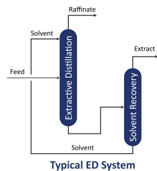
Typical ED System
